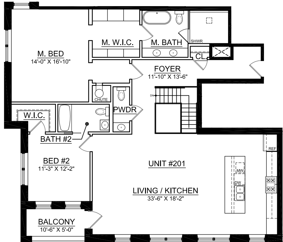
UNIT 201 - 2ND FLOOR SCALE: 1/8" = 1'-0" DUPLEX UP TOWNHOME UNIT
