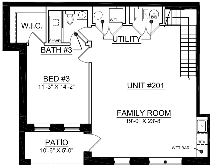
UNIT 201 - MAIN FLOOR SCALE: 1/8" = 1'-0" DUPLEX UP TOWNHOME UNIT
